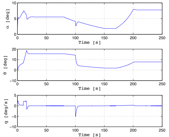
Fig. 5. Time evolution of the angles of attack \alpha and pitch \theta , and the angular velocity q .
