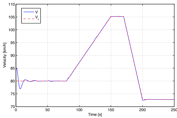
Fig. 2. Time evolution of the aerodynamic velocity (solid), compared with its reference (dashed).
