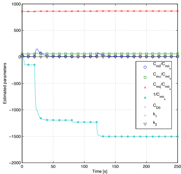
Fig. 6. Time evolution of the estimated parameters and aerodynamic coefficients, showing convergence to some values.
