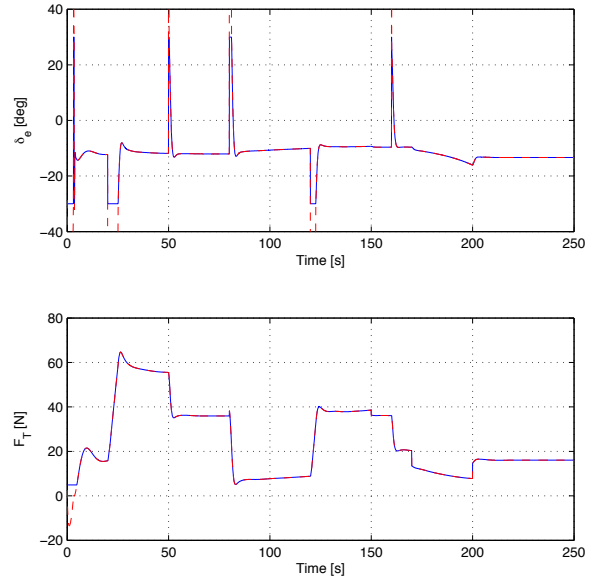
Fig. 4. Control signals: computed (dashed) and commanded (solid), which includes saturation.
