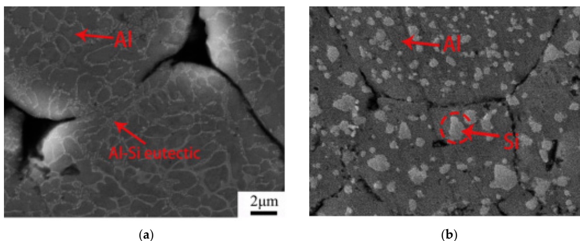
Figure 11. Consolidation of Al-12Si powders: (a) by EDC, with the original eutectic structure being maintained; (b) by spark plasma sintering (SPS), with the original microstructure being changed. Reprinted with permission from ref. [77] Copyright 2020 Elsevier.
