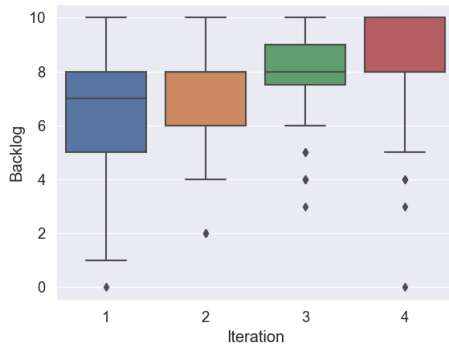
Figure 3: Self-assessment results on backlog delivery practices.
