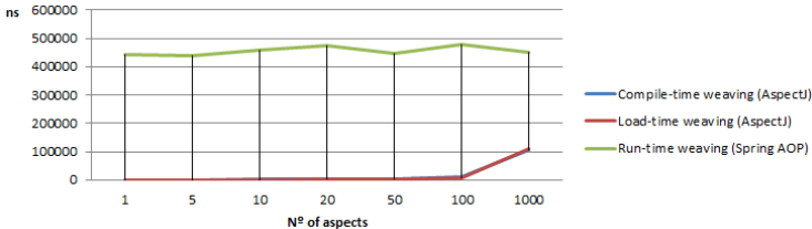
Fig. 6. Aspect weavers performance: aspects execution time
