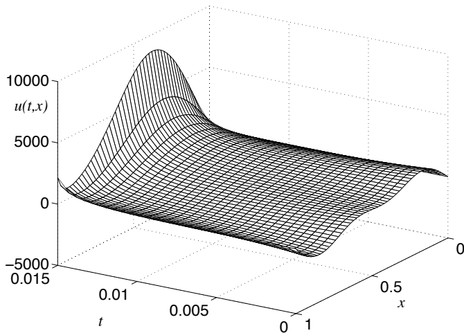
Fig. 5. Closed-loop simulation for u(t, x) using only the first (linear) order kernel k_1 , in the example of Section 3.1.
