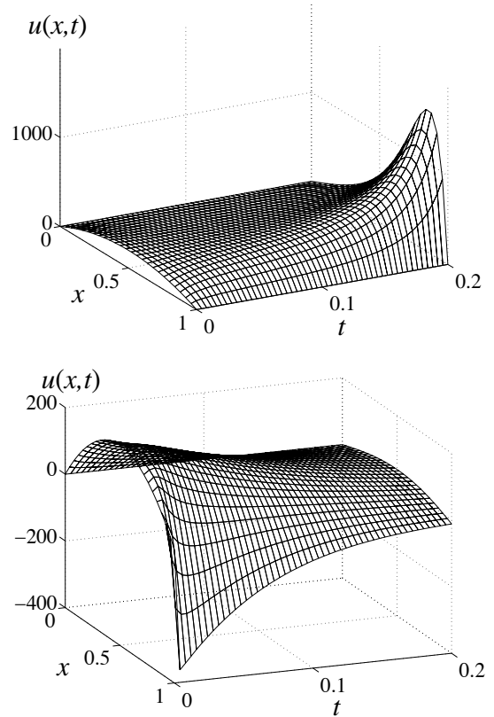
Fig. 3. Uncontrolled (left) and controlled system (right) for the example of Section 5. The solution of the uncontrolled system blows up in finite time. The trajectory of the control input (right) is u(t, 1) . The size of the control effort (-400) is reasonable given the size of the initial condition (with a peak about 200).
