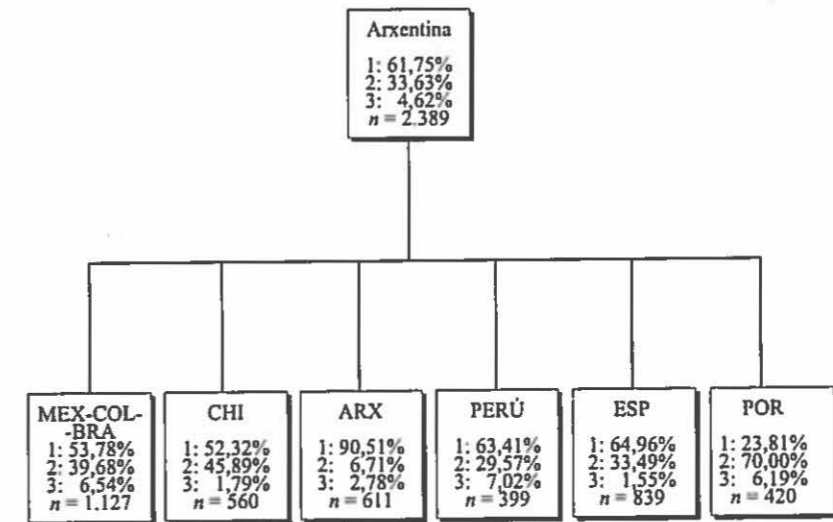
Figura 4.- Chi-Squared Automatic Interaction Detector (CHAID)
