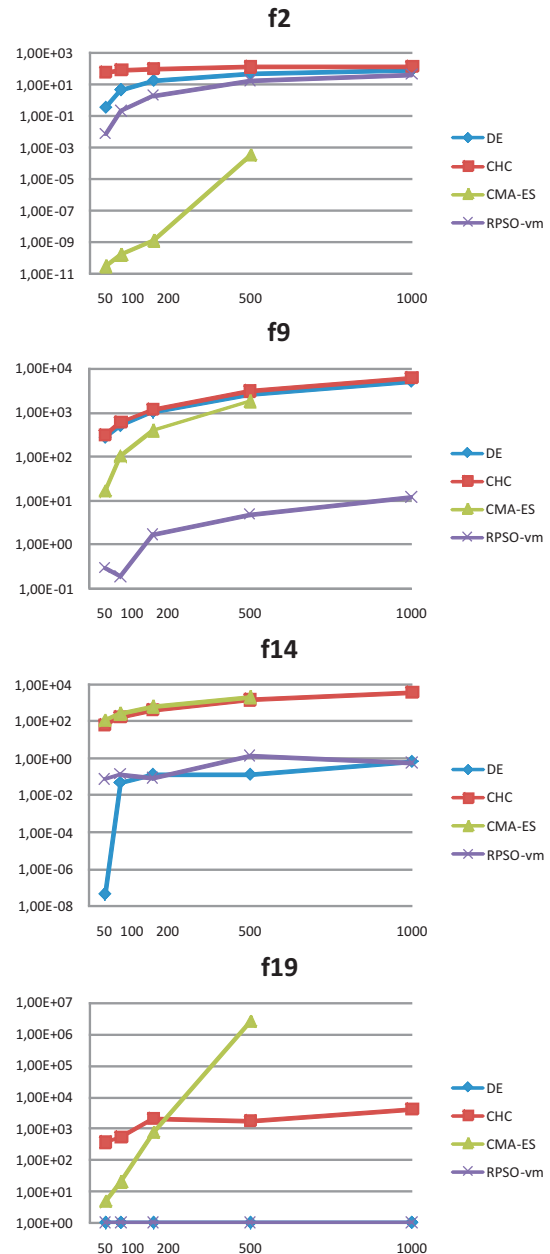
Fig. 1 Scalable results of DE, CHC, G-CMA-ES, and RPSO-vm for functions f2, f9, f14, and f19. Y axis shows the results in logarithmic scale. X axis shows the problem dimensions
