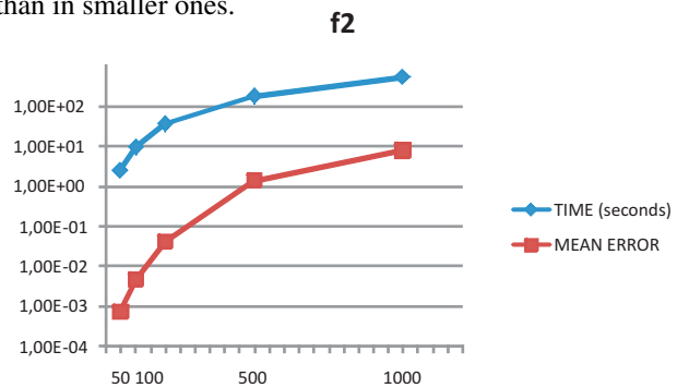
Fig. 2 Differences in times versus mean error magnitudes of f2 for each dimension. Y axis contains values in logarithmic scale and X axis contains dimensions
