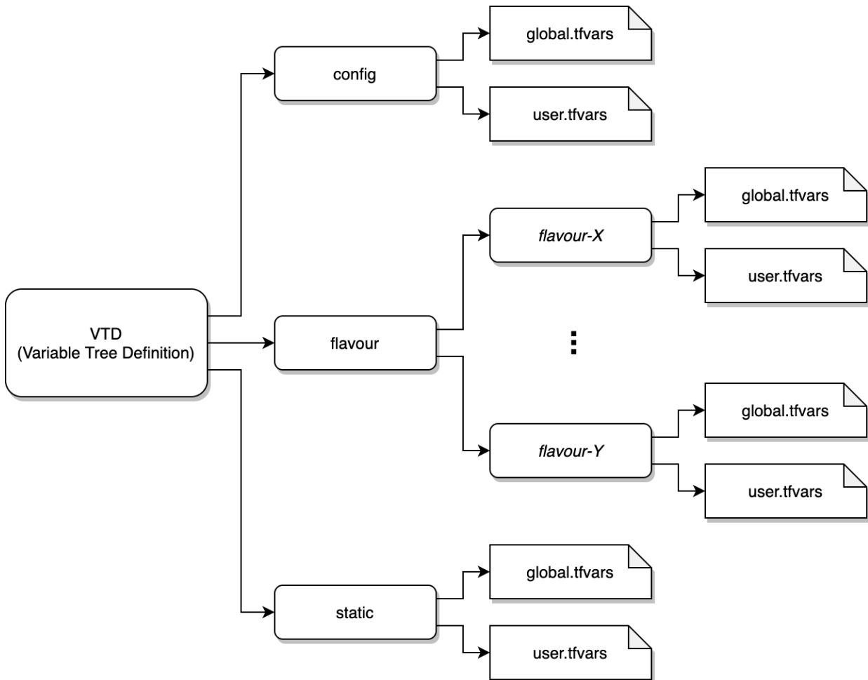
Figura 2 VTD: Variable Tree Definition
