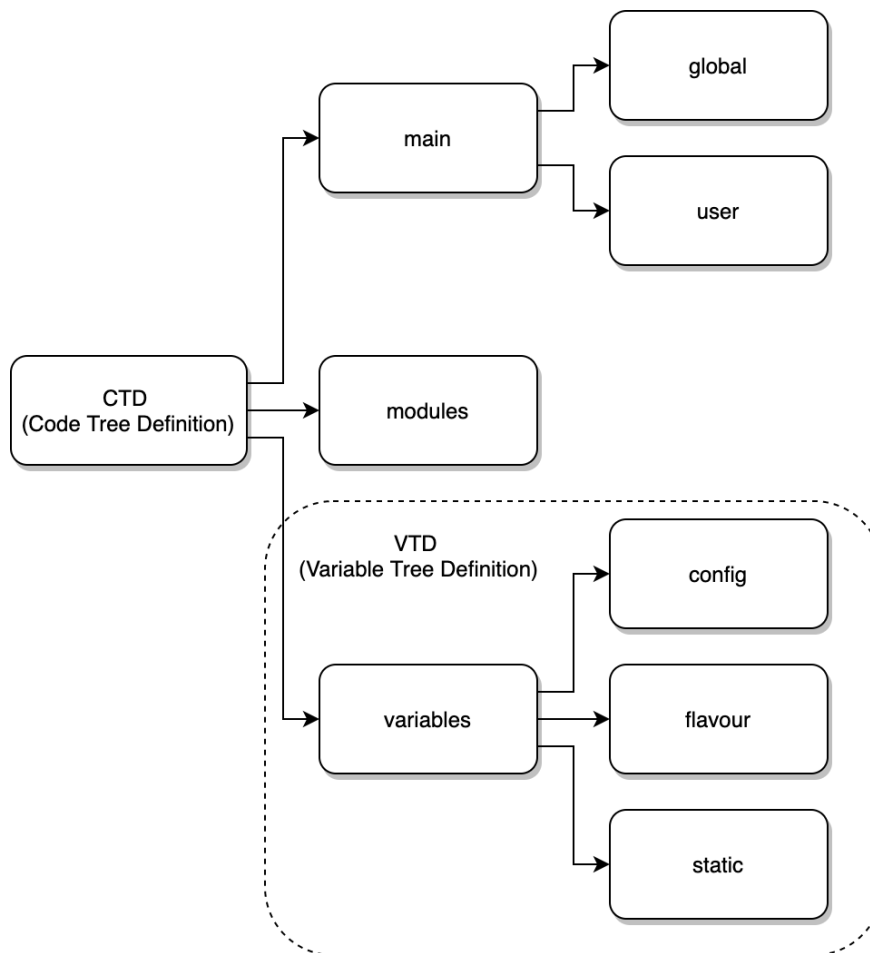
Figura 1 CTD: Code Tree Definition
