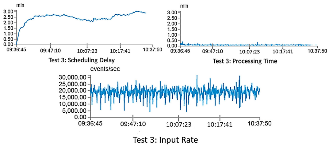
Fig. 10. Test 3. Scheduling delay, processing time, and input data during execution.
