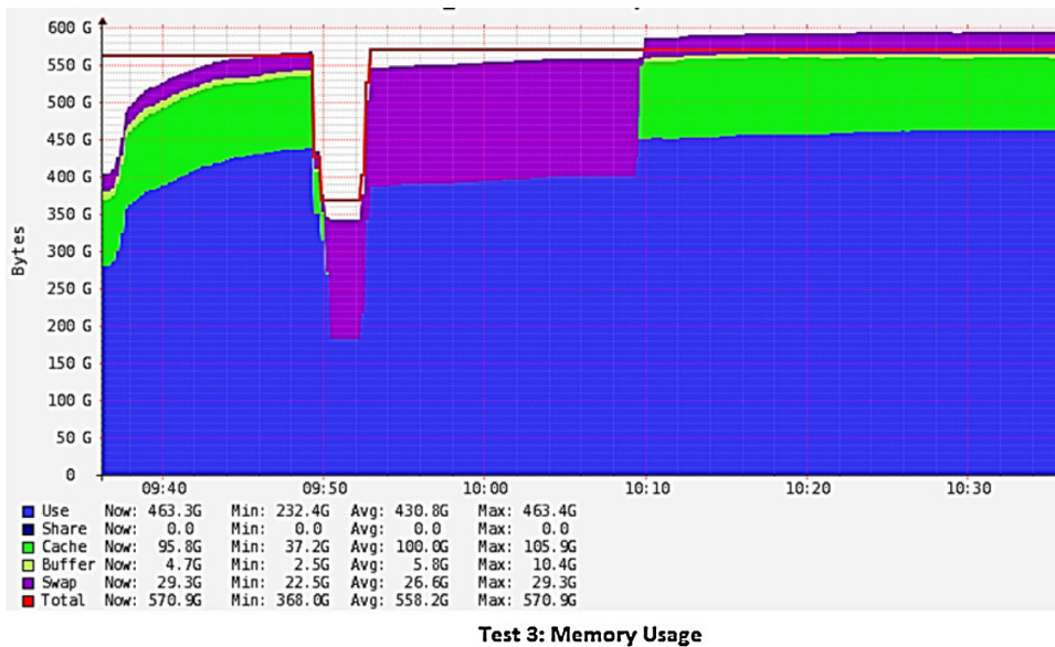
Fig. 12. Test 3. Memory usage level.
