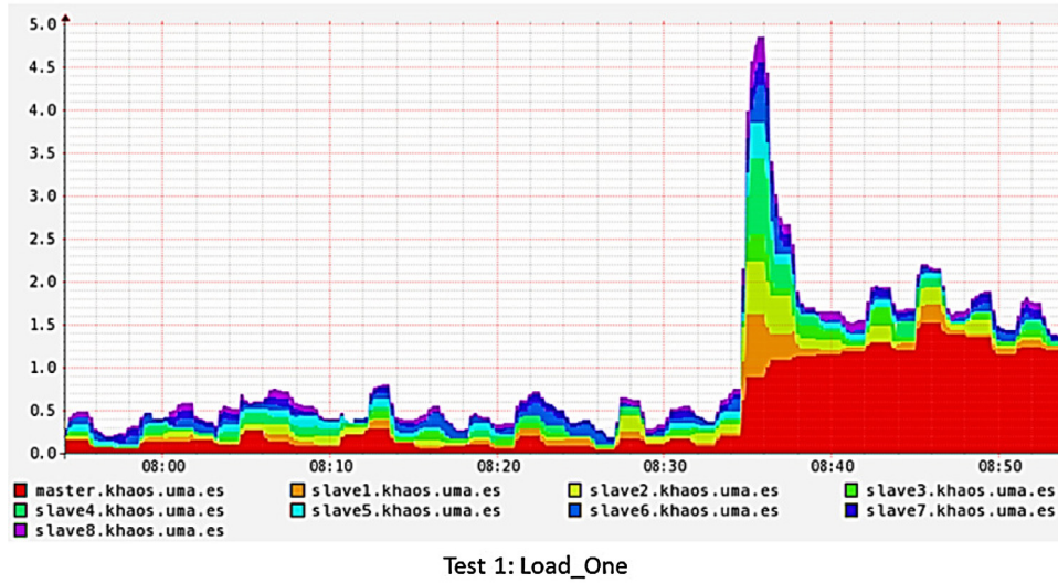
Fig. 5. Test 1. Load.one. Number of threads per node.
