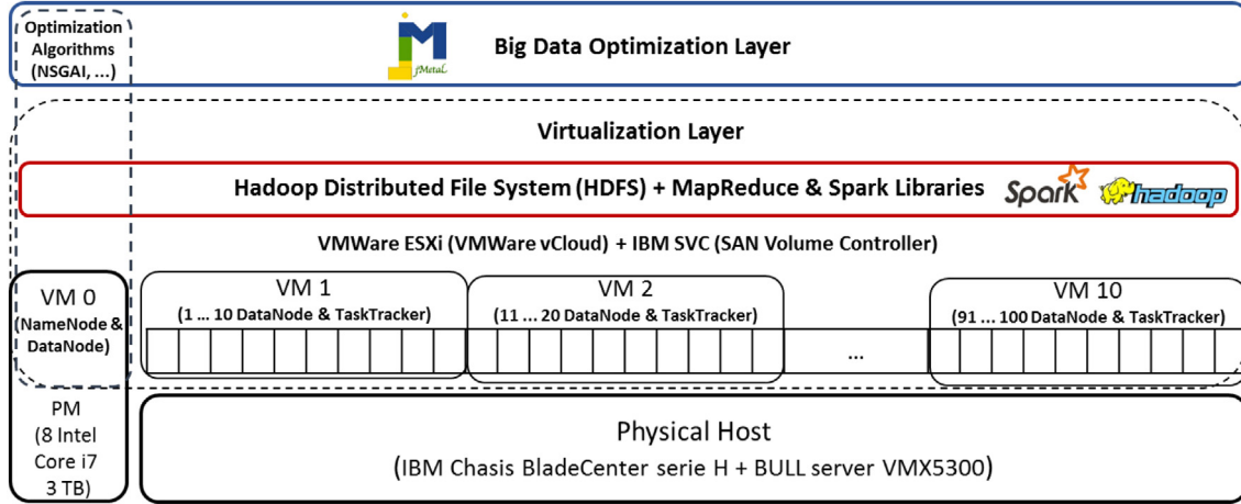
Fig. 3. Computational environment for Big Data optimization used to test the performance of jMetal-Spark under different conditions of computational effort and big data management.
