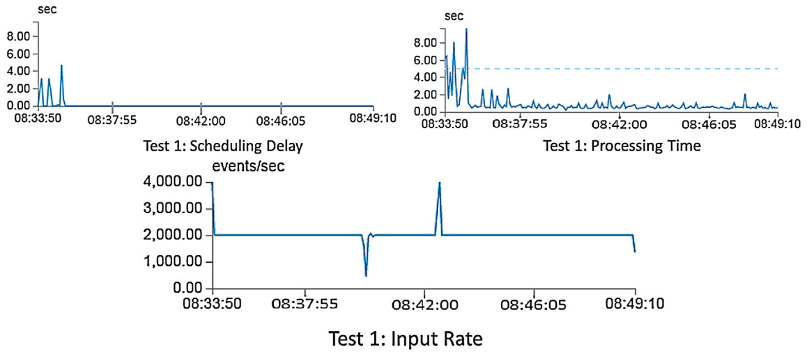
Fig. 4. Test 1. Scheduling delay, processing time, and input data during execution.
