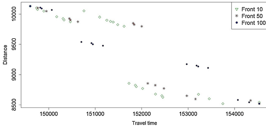
Fig. 14. Pareto front approximations obtained when solving the DTSP of New York with Dynamic MOCeL.
