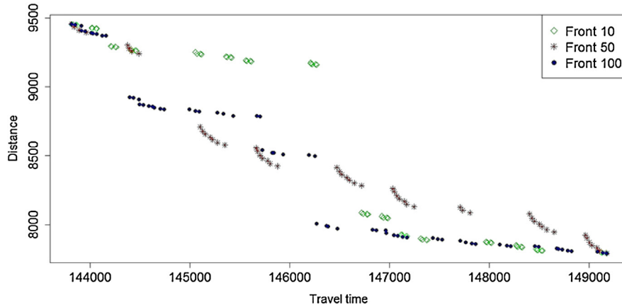
Fig. 13. Pareto front approximations obtained when solving the DTSP of New York with Dynamic NSGAI.
