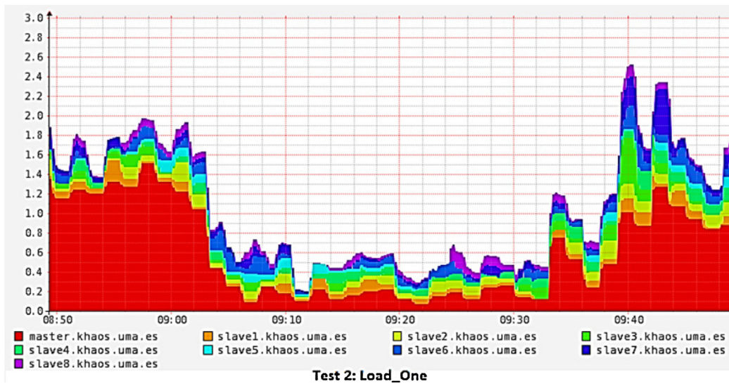
Fig. 8. Test 2. Load.one. Number of thread per node.
