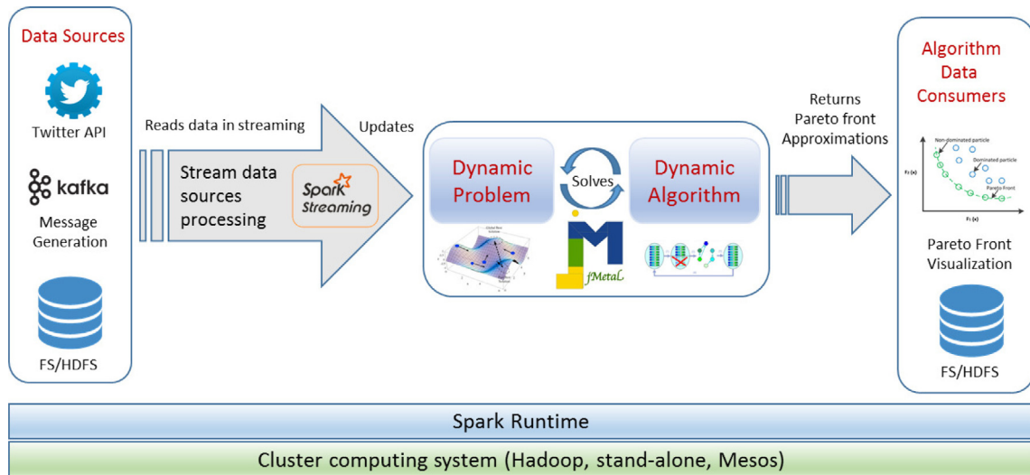
Fig. 1. Architecture overview of jMetalSP.
