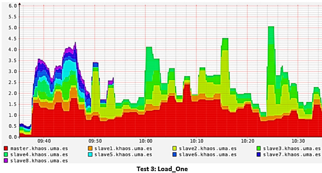
Fig. 11. Test 3. Load.one. Number of threads per node.
