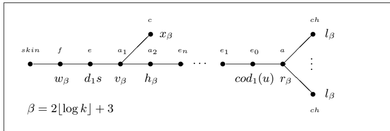
Fig. 2. TIME 2\lceil \log k \rceil + 3
