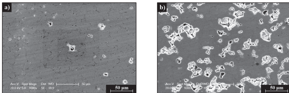
Figure 4. Distribution of porosity (SEM) in \text{Al}_{50}\text{Ti}_{50} compact ERS7/40. (a) Core and (b) periphery of the compact.
