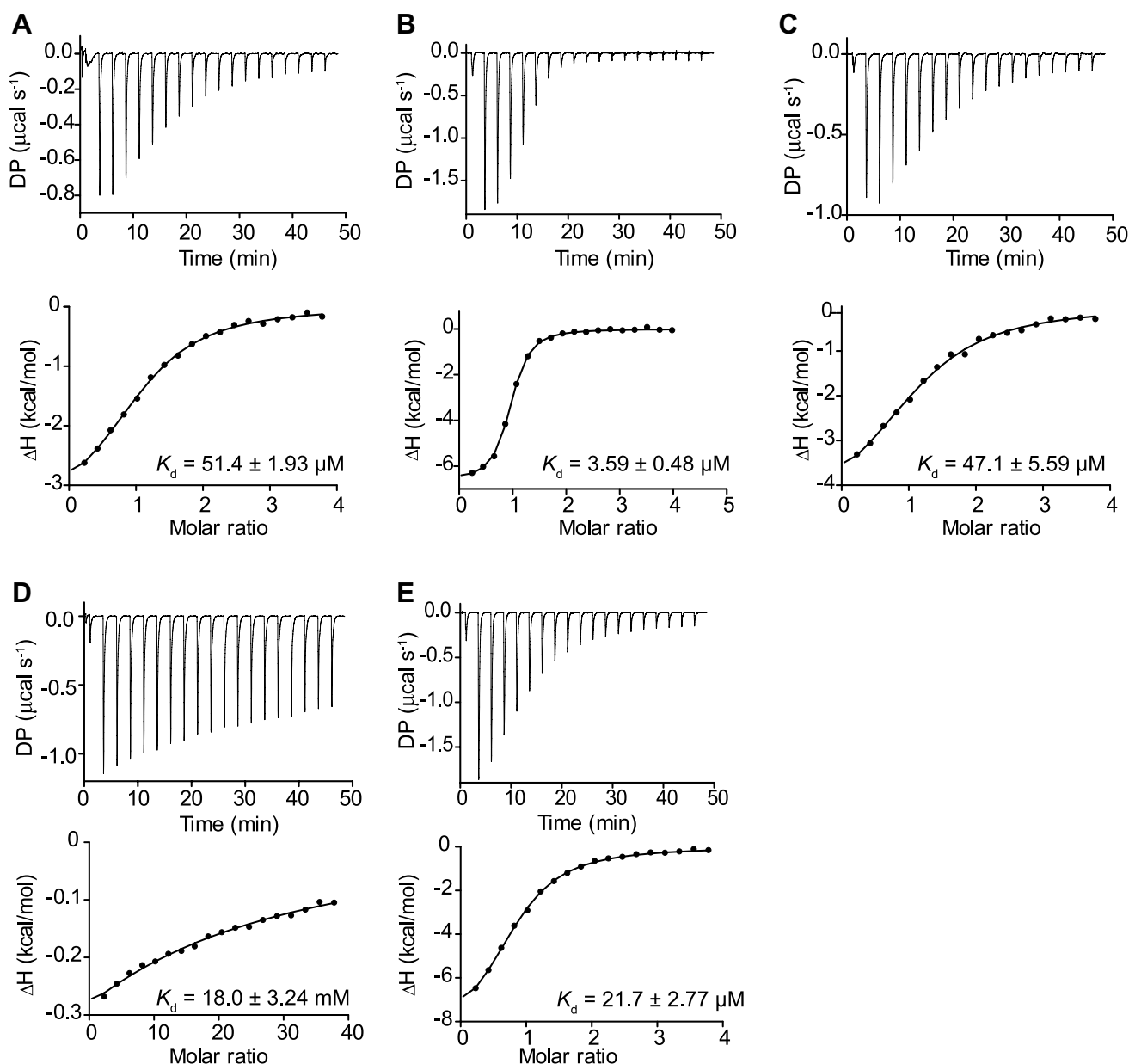
Fig. 5 ITC isotherms of R. gnavus GH29 fucosidase E1_10125 binding to fucosylated ligands. a E1_10125 binding to LeX. b E1_10125 binding to sLeX. c E1_10125 binding to \alpha\text{Gal-LeX} . d E1_10125 binding to Neu5Ac. e E1_10125 binding to L-Fucose. DP differential power
