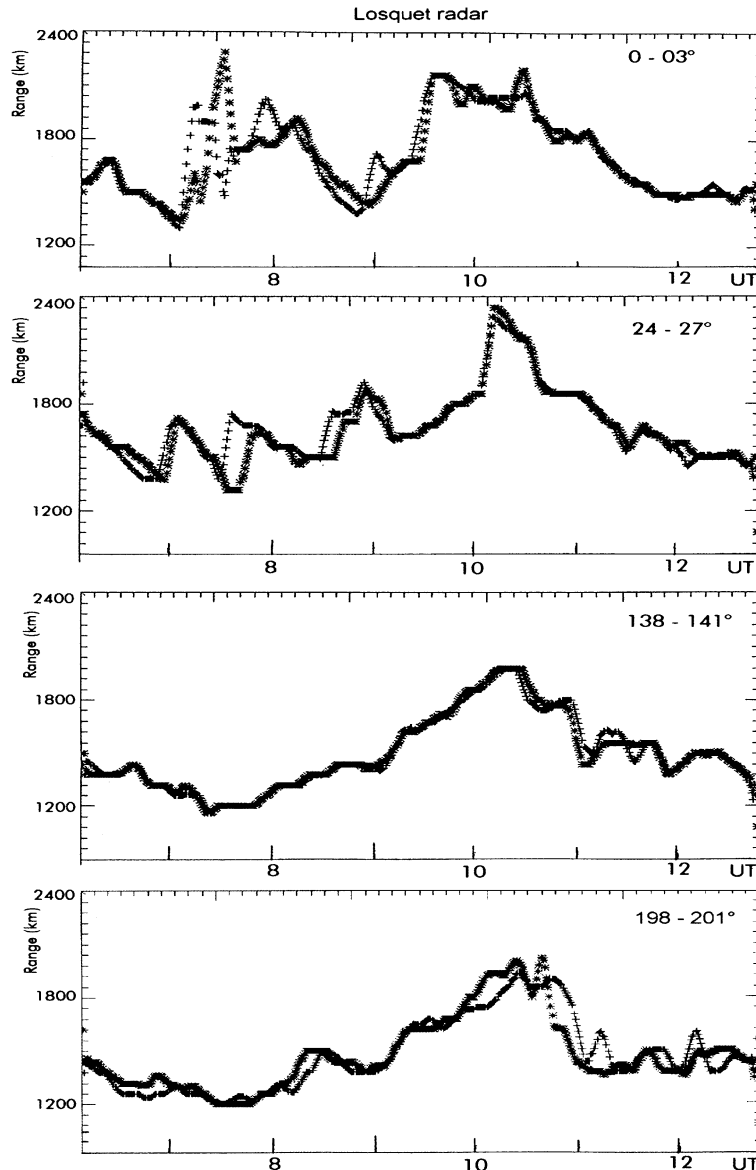
Fig. 2. Return group path versus UT from Losquet Island (Lannion) in four different azimuths: 0-3^\circ , top panel; 24-27^\circ , second panel; 138-141^\circ , third panel and 198-201^\circ , bottom panel.
