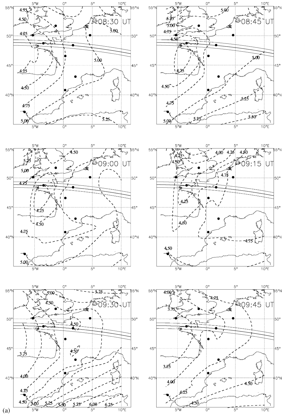
Fig. 4. Contour maps of foF1 quarter-hourly values between 0830 and 1045 UT and between 1200 and 1300 UT drawn on a 50 \times 50 km grid. An open circle is drawn on the eclipse path when the Moon shadow is projected on the ionosphere (at 1015 and 1030 UT) at 200 km height above Western Europe.
