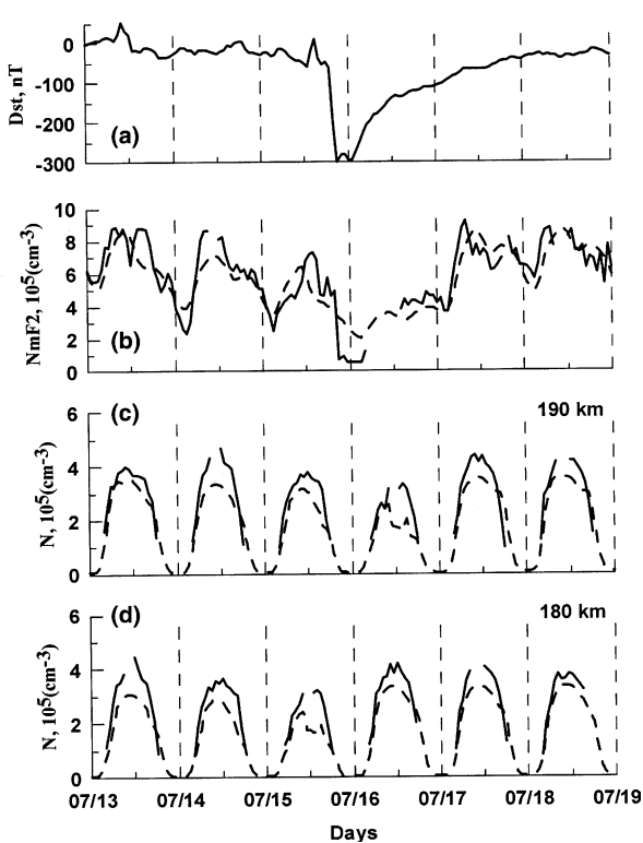
Fig. 9. Superstorm of July 2000: (a) hourly Dst indices, (b) measured and IRI model predicted N_mF2 values for Pruhonice, (c) measured and IRI-predicted electron density courses at 190 km for Pruhonice, (d) the same for 180 km. The observed values are shown as solid lines. The IRI model values are shown as dash lines. Time is in UT.
