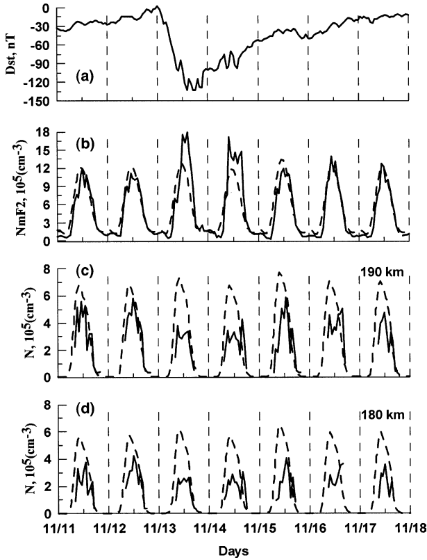
Fig. 7. Storm of November 1998: (a) hourly Dst indices, (b) measured and IRI model predicted N_mF2 values for Pruhonice, (c) measured and IRI-predicted electron density courses at 190 km for Pruhonice, (d) the same for 180 km. The observed values are shown as solid lines. The IRI model values are shown as dash lines. Time is in UT.
