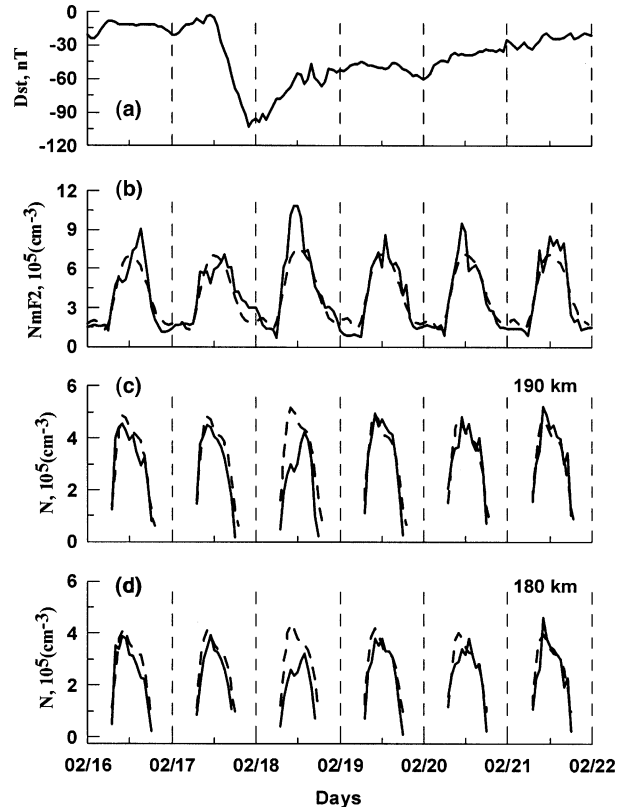
Fig. 6. Storm of February 1998: (a) hourly Dst indices, (b) measured and IRI model predicted N_mF2 values for Ebro, (c) measured and IRI-predicted electron density courses at 190 km for Ebro, (d) the same for 180 km. The observed values are shown as solid lines. The IRI model values are shown as dash lines. Time is in UT.
