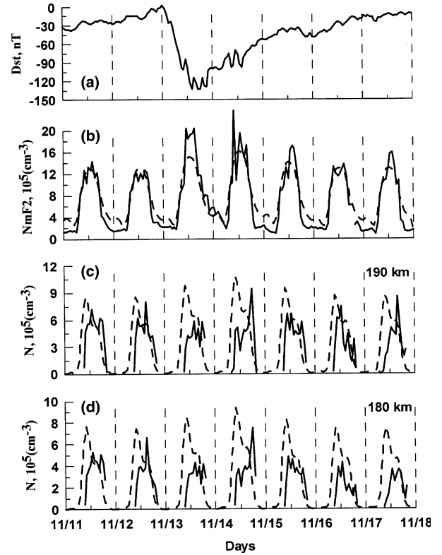
Fig. 8. Storm of November 1998: (a) hourly Dst indices, (b) measured and IRI model predicted N_mF2 values for Arenosillo, (c) measured and IRI-predicted electron density courses at 190 km for Arenosillo, (d) the same for 180 km. The observed values are shown as solid lines. The IRI model values are shown as dash lines. Time is in UT.
