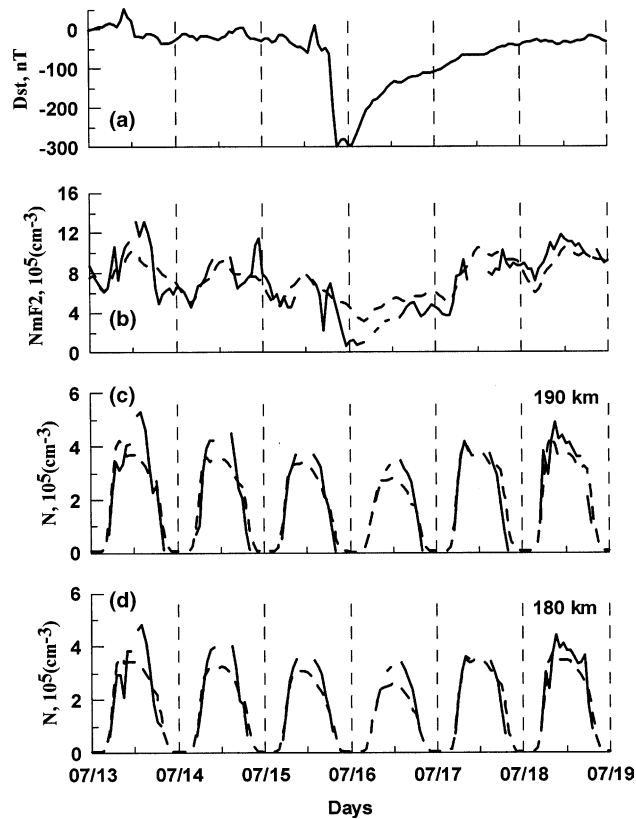
Fig. 10. Superstorm of July 2000: (a) hourly Dst indices, (b) measured and IRI model predicted N_mF2 values for Ebro, (c) measured and IRI-predicted electron density courses at 190 km for Ebro, (d) the same for 180 km. The observed values are shown as solid lines. The IRI model values are shown as dash lines. Time is in UT.
