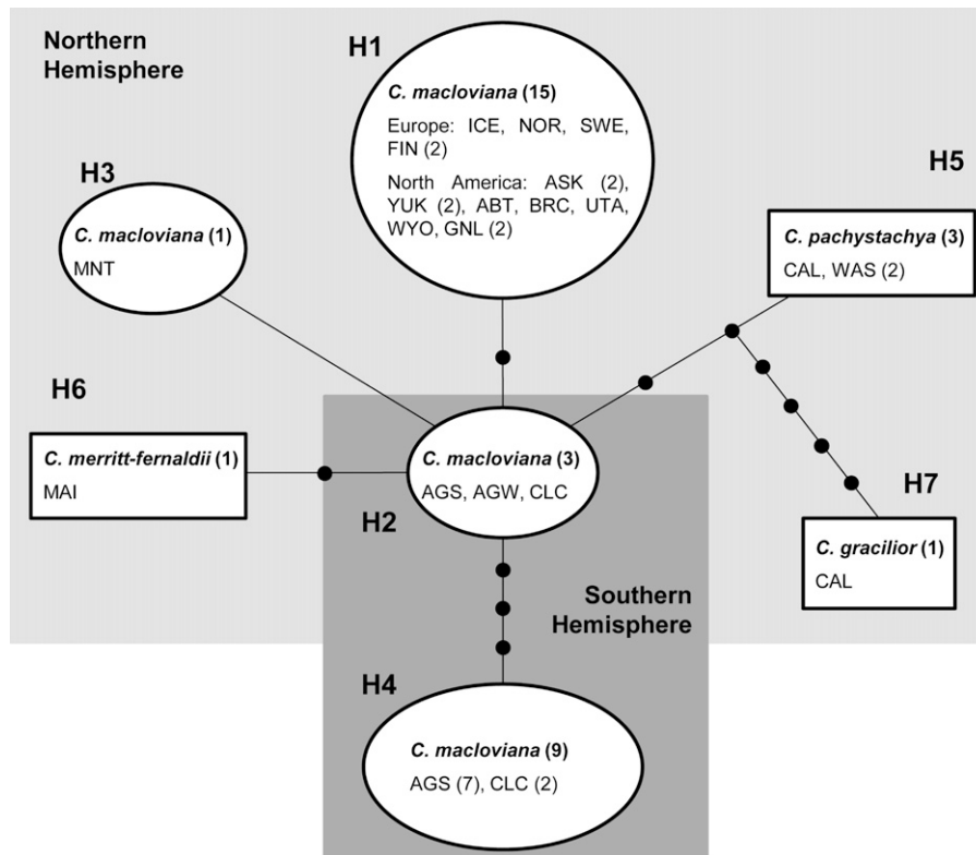
FIGURE 3 Plastid DNA haplotype network ( rps16 , 5'trnK , and psbA-trnH ) with coded indels. Circles represent C. macloviana sampled haplotypes (H1–H4), squares represent ingroup sampled haplotypes (H5–H7), lines depict single mutational steps, and black circles correspond to not sampled or extinct haplotypes.
