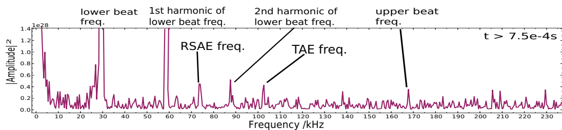
(b) FFT of losses' time signal during stochastic phase
