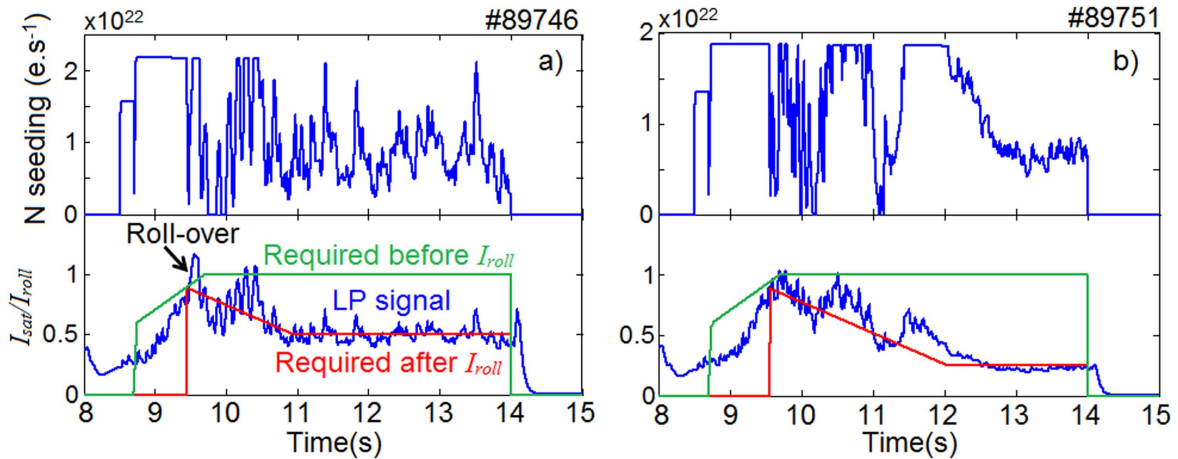
Figure 5. (a) Top: N injection rate time trace. Bottom: real-time attachment fraction time trace (blue curve) with pre-roll-over request (green curve) and post-roll-over request (red curve) for discharge #89 746. (b) Same as (a) for discharge #89 751.
