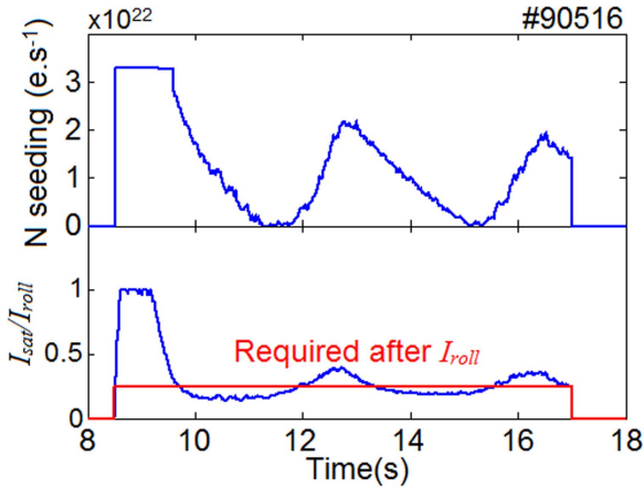
Figure 7. Same as figure 6 for discharge #90 516. No pre-roll-over request was necessary since the controller was using the automatic roll-over search feature.
