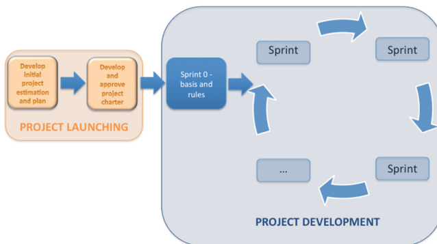
Fig. 2. NDT-Agile lifecycle [35]
