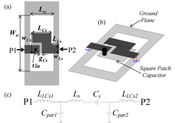
Fig. 5. (a) Top view, (b) 3-D view, and (c) lumped-element equivalent-circuit model of the series branches of the proposed balanced UWB bandpass filter. Dimensions are W_w = 3.3 mm, L_w = 1.46 mm, w_{L_s} = 0.5 mm, L_{L_s} = 0.49 mm, w_{C_s} = 1.22 mm, L_{C_s} = 1.2 mm, and g_{C_s} = 0.144 mm.
