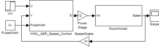
Fig. 4 Motor simulation model
