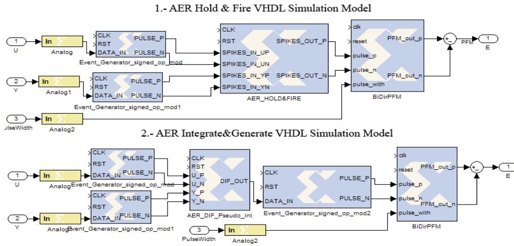
Fig. 6 VHDL blocks for simulation
