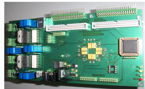
Fig. 7 AER-Robot board photograph
