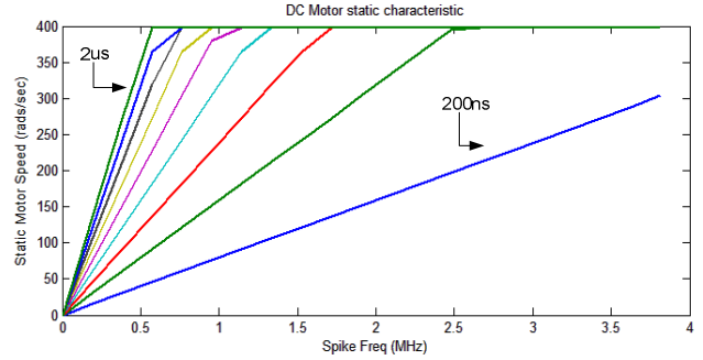
Fig. 3 Static speed characteristic of a DC motor using a PFM scheme
