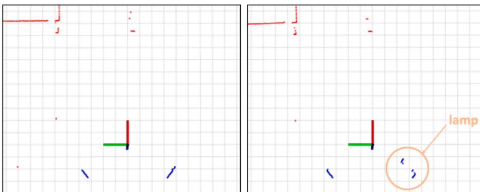
Fig. 5. Layout of the split 2D LiDAR scan. The red points represent LiDAR measurements in the horizontal plane (caused by walls and beams), while the blue points correspond to LiDAR measurements in the vertical plane. Two cases are shown: left) the vertical segments of both mirrors measure robot-ceiling distances, and right) one vertical segment measures robot-ceiling distance while the other contains points partially reflected by a lamp. (For interpretation of the references to colour in this figure legend, the reader is referred to the web version of this article.)
