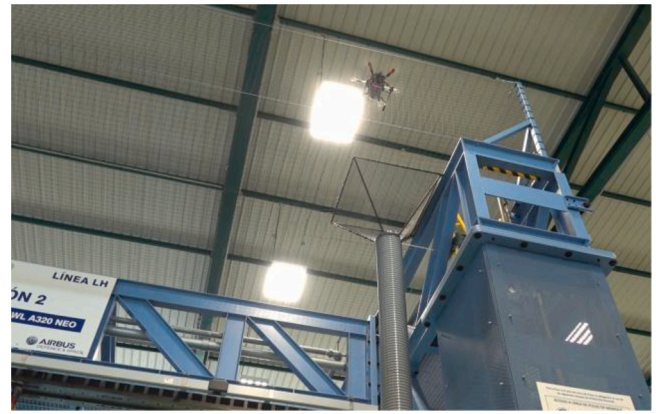
Fig. 6. Light object logistics delivery point, with the aerial robot positioned right before releasing the requested component.
