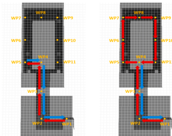
Fig. 7. Layout of the factory with the selected navigation waypoints (in orange) and sample trajectories for the two missions: light object logistics (left) and missing tool search (right).
