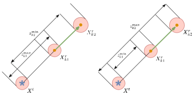
Fig. 8. Robot moving straight away from the tool (from X_{k_1}^r to X_{k_2}^r ). The red circles represent the 3\sigma_k^r uncertainty of the robot's positions (orange dots) and the radio range measurements (depicted as uncertainty around the real tool position X^t at the blue asterisk): left) case of minimum difference between inlier measurements; and right) case of maximum difference between inlier measurements. (For interpretation of the references to colour in this figure legend, the reader is referred to the web version of this article.)
