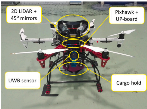
Fig. 3. Closeup picture of the developed aerial system.
