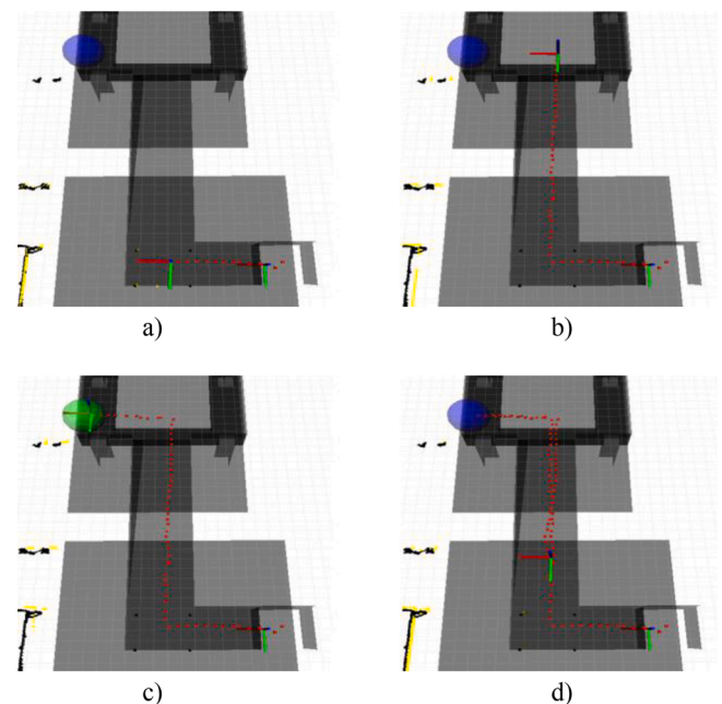
Fig. 11. Light object delivery experiment: a) the robot takes off ; and navigates through the vertical and horizontal ducts following waypoints WP1 and WP2 ; b) the robot continues to waypoints WP3 and WP4 ; c) the robot reaches WP5 (location of delivery point A) and opens the cargo hold to release the requested component, and; d) the robot returns following the same path towards the logistics area.
