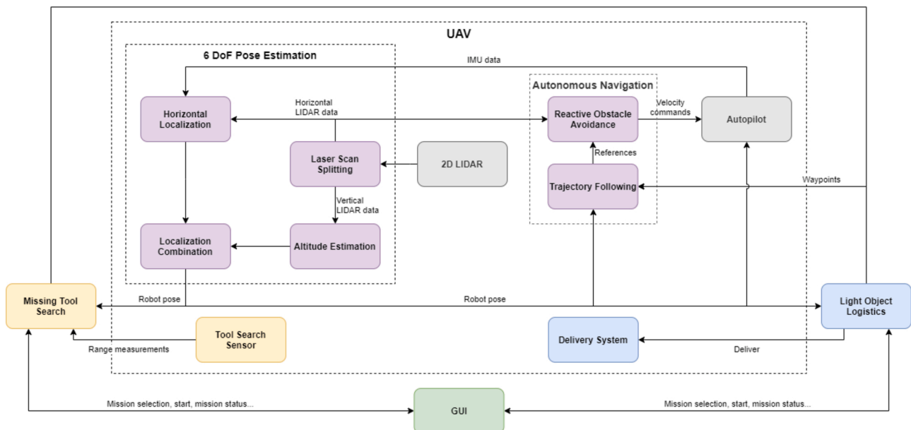
Fig. 4. Functional architecture of the proposed system.
