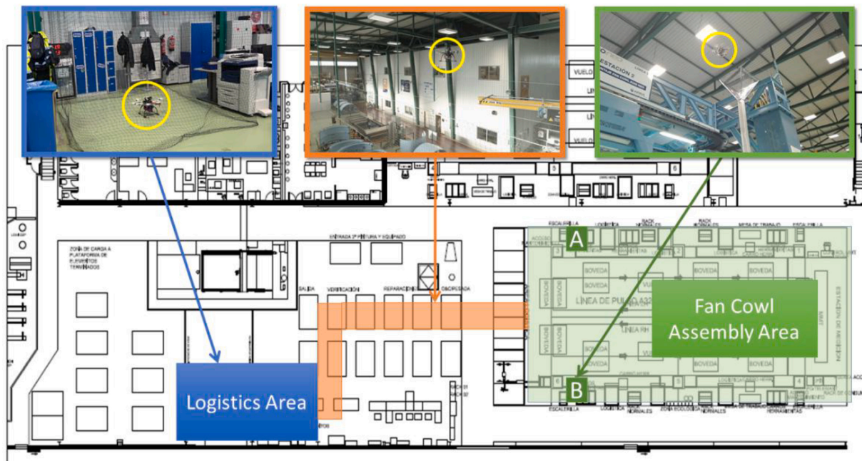
Fig. 10. Layout of the CBC Airbus D&S factory showing the storage center at the logistics area with the take-off ;/landing location (in blue), the flying corridor (in orange) towards the fan cowl assembly working area (in light green), which includes hoppers A and B for light object delivery (in dark green). (For interpretation of the references to colour in this figure legend, the reader is referred to the web version of this article.)
