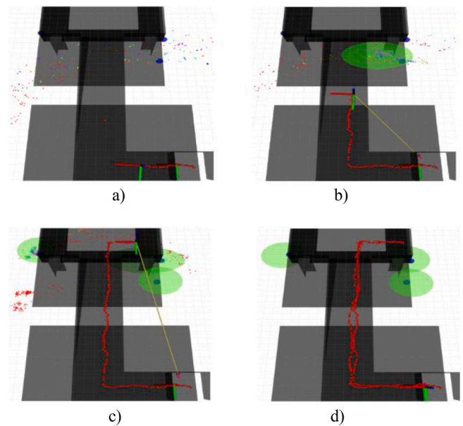
Fig. 12. Missing tool search experiment while the robot performs light object logistics tasks. The tool ground-truth locations are depicted as blue spheres. The PFs particles are depicted as colored dots, scaled from blue (higher particle weights) to red (lower weights). The uncertainty regions with radii lower than 3 m are shown as green ellipsoids. (For interpretation of the references to colour in this figure legend, the reader is referred to the web version of this article.)
