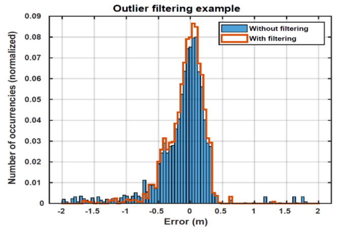
Fig. 9. Histogram of UWB measurement errors in one experiment in the factory before (in blue) and after (in red) outlier filtering. (For interpretation of the references to colour in this figure legend, the reader is referred to the web version of this article.)
