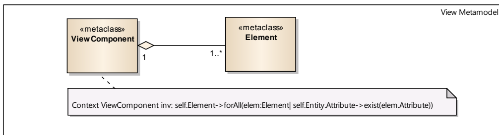
Fig 5. View Component Metamodel Section
