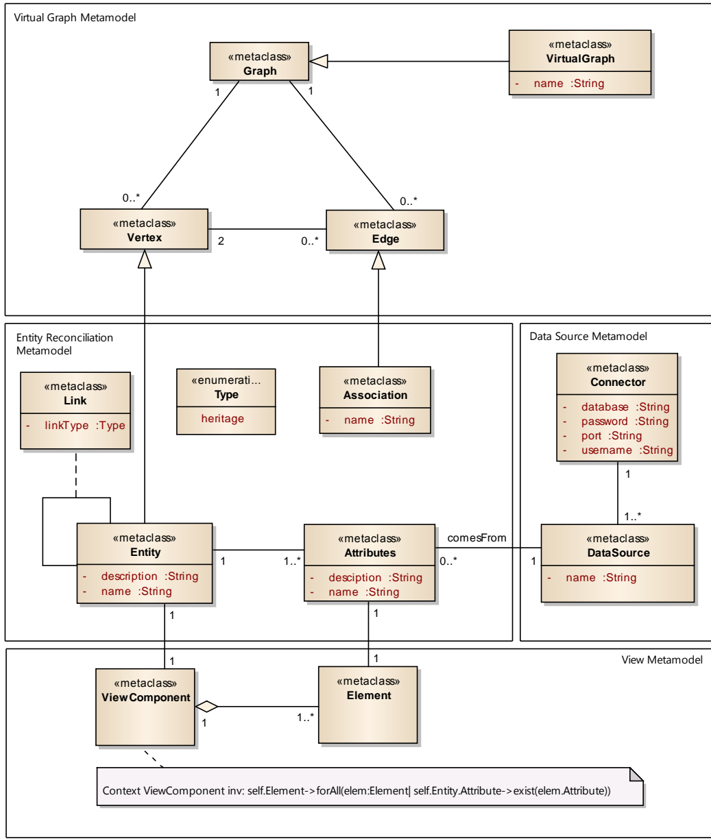
Fig 1. Metamodel for solving the ER problem
