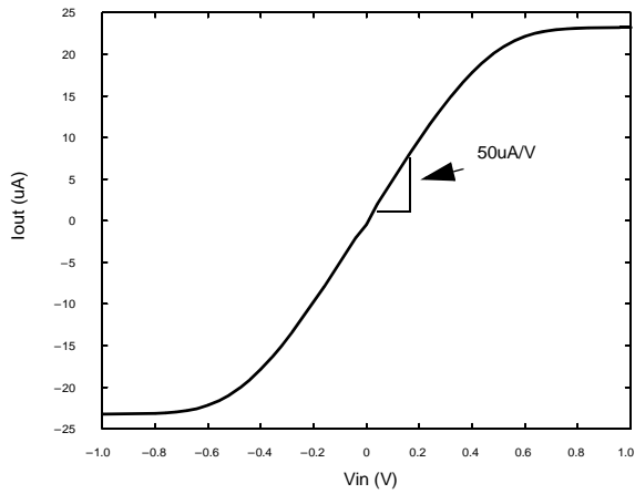
Figure 9 :Input/output characteristic of the unitary transconductor of value 50uA/V.
