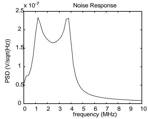
Figure 13 :Output Power Spectral Density.
