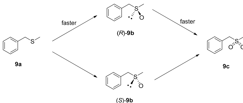
Scheme 2. PockeMO-catalyzed sulfoxidation of benzyl methyl sulfide 9a in 50 mM Tris/HCl (pH 8.0) containing 10% v v -1 1,4-dioxane.
