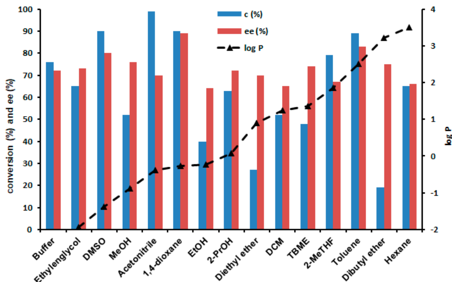
Figure 3. Effect of different organic solvents (10% v v^{-1} ) on the conversion and the stereoselectivity of the enzymatic sulfoxidation of 2a catalyzed by PockeMO. Reactions were performed at 25 °C for 24 h. log P (▲) values are plotted as reference for the hydrophobicity of the solvent. DMSO: Dimethylsulfoxide; MeOH: Methanol; EtOH: Ethanol; 2-PrOH: 2-Propanol; TBME: tert -butyl methyl ether; DCM: Dichloromethane; 2-MeTHF: 2-Methyltetrahydrofuran.
