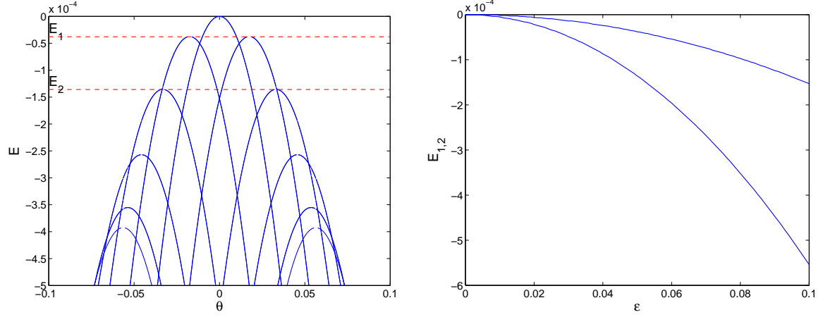
Figure 14. Phonobreather in a \phi^4 potential with \omega_b = 2 , \alpha = \pi/2 and N = 20 . (Left) Band diagram for \epsilon = 0.05 . (Right) Dependence of the location of the maxima of the two bands closest to E = 0 with respect to \epsilon .
