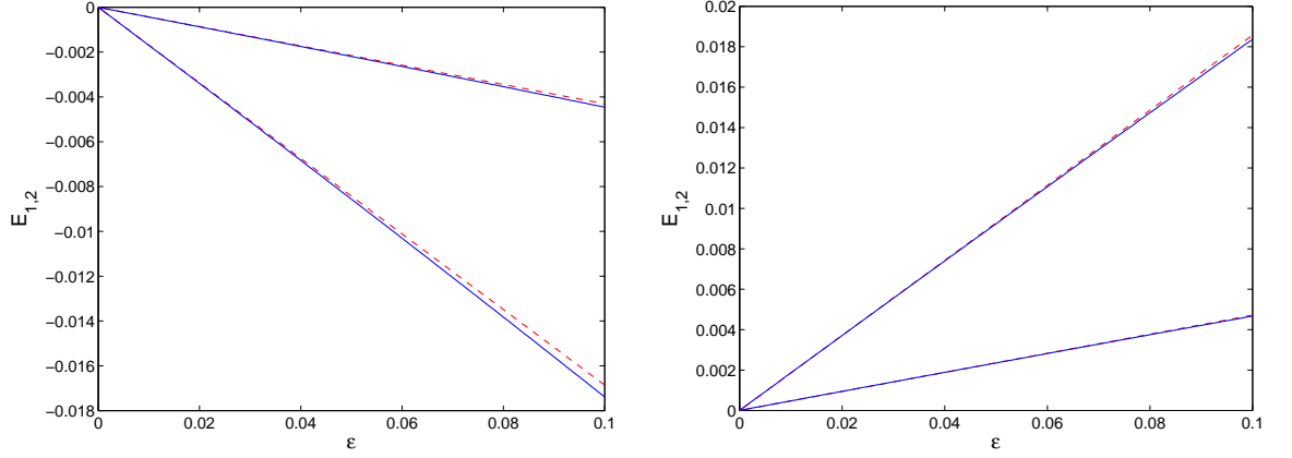
Figure 13. Dependence of the location of the maxima of the two bands closest to E = 0 (represented by E_1 and E_2 ) with respect to \epsilon for phonobreaters in a \phi^4 with \alpha = 2\pi/3 , N = 21 (left) and \alpha = \pi/4 , N = 24 (right). In both cases, \omega_b = 0.8 . Dashed lines correspond to the MST predictions and full lines to the numerical values. Dashed lines correspond to the MST predictions and full lines to the numerical values.
