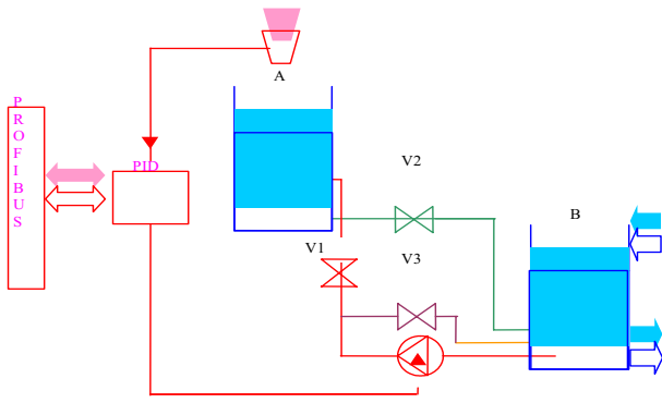
Figure 12: Laboratory plant
