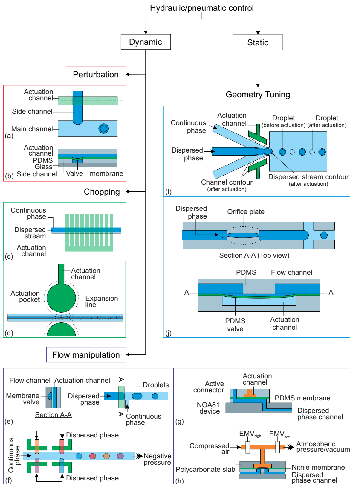
Fig. 5 Classification of the hydraulic/pneumatic control approaches. (a) T-junction with actuation channel 92 (b) Side view along the actuation channel (dashed line); (c) Actuation channels connected to 10 valves which are used to chop the dispersed stream into individual droplets 93 (d) Horizontal moving valve connected to actuation channel; 94 (e) On demand droplet generation using rounded profile T-junction channel and membrane valve; 95 (f) Multiples of T-junctions to produce droplets with distinct composition; 96 (g) Stiff NOA81 device with active connector; 97 (h) Polycarbonate slabs with nitrile membrane; 98 (i) A valve is actuated by expanding the actuation channel pneumatically. This reduces the channel size around the orifice and obstructs the dispersed phase stream, resulting in a reduction of the droplet size; 99 (j) Integrated adjustable orifice plate at the dispersed phase channel. The dotted lines illustrate the changes after activation of the hydraulic/pneumatic control. 100
