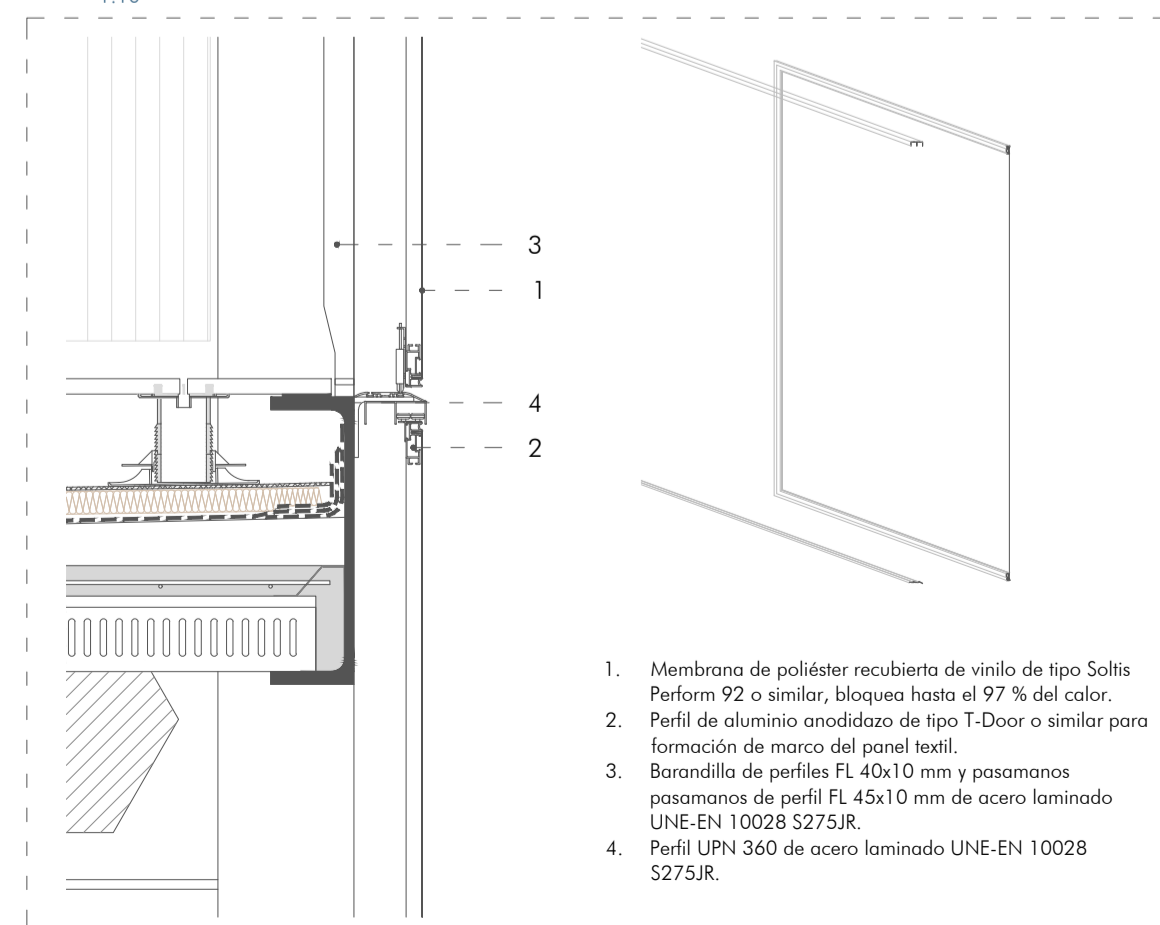
Panel Textil Deslizante 1:10
